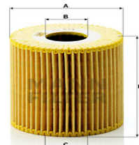
Oil Filter HU 819 x EM-10147
