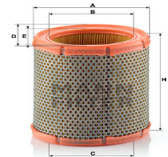
Air Filters C 1460 EM-30347
