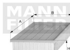
Air Filters C 25 131 EM-30013
