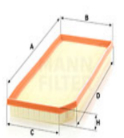
Air Filters C 41 002 EM-30097
