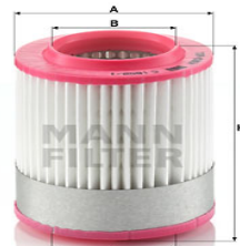
Air Filters C 1652/1 EM-30123
