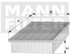
Air Filters C 23 906 EM-30160
