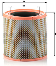
Air Filters C 1380/3 EM-30361
