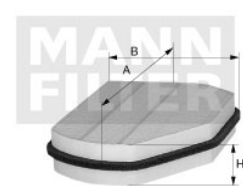
Air Filters C 24 009 EM-30031
