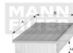
Air Filters C 29 009 EM-30075
